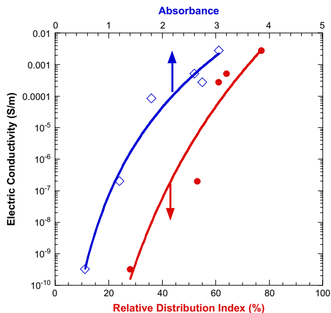
Fig. 12. The relationships between electric conductivity of PMMA/SWNT (0.5%) and electrical conductivity and quantitative dispersion levels of SWNT described with relative dispersion index (0.1 \mu\text{m} , 1 \mu\text{m}^3 , 84,640 \mu\text{m}^3 , 1) (solid circles) and with absorbance at 275 nm (open squares). Power fits and correlation coefficient, R , with RDI is 0.99 and that with absorbance is 0.96.
