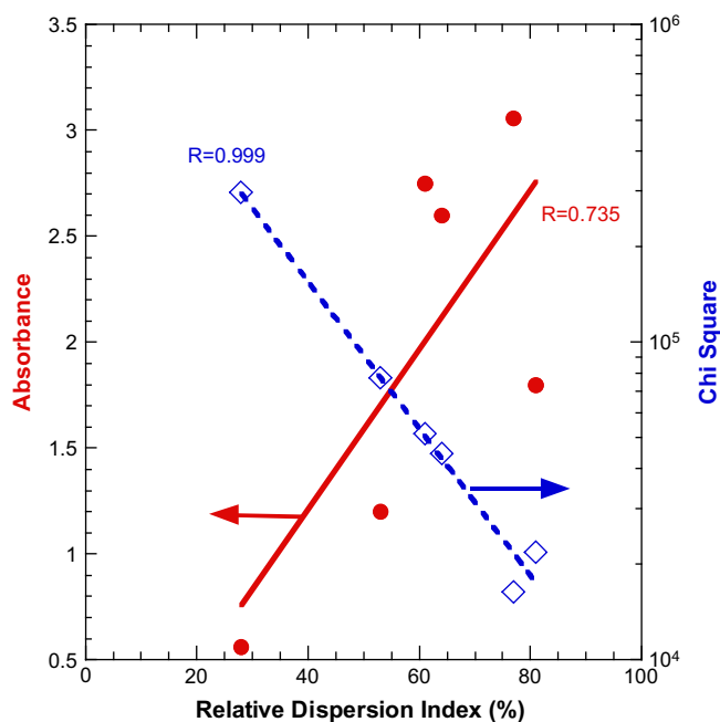
Fig. 6. Relationship between relative dispersion index ( 0.1 \mu\text{m} , 1 \mu\text{m}^3 , 84,640 \mu\text{m}^3 , 1), \chi^2 ( 0.1 \mu\text{m} , 1 \mu\text{m}^3 , 84,640 \mu\text{m}^3 , 1) with open squares, and absorbance at 275 nm with solid circles. R is correlation coefficient.
