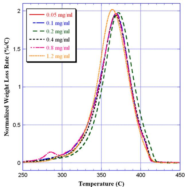
Fig. 7. DTG, dynamic thermogravimetric, curves of the six PMMA/SWNT (0.5%) nanocomposites prepared by different SWNT concentrations in DMF. TGA was conducted in nitrogen at heating rate of 5^\circ\text{C}/\text{min} .
